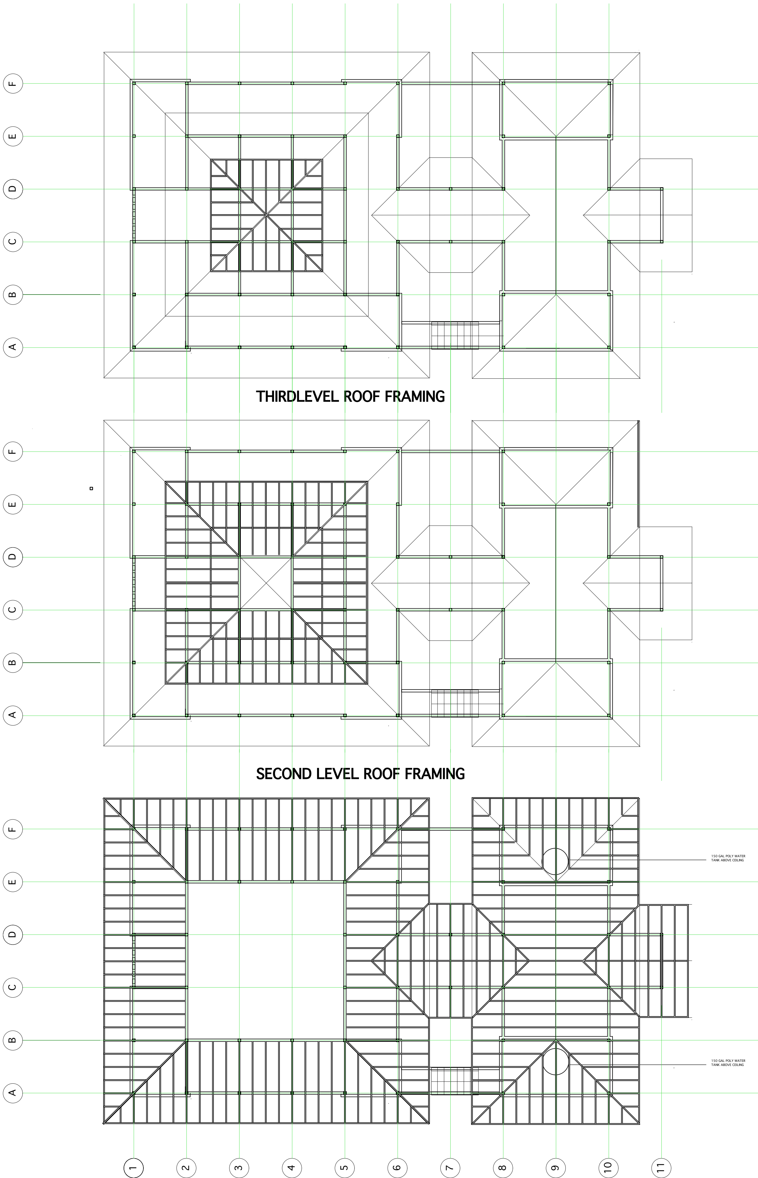
FIRST LEVEL ROOF FRAMING
